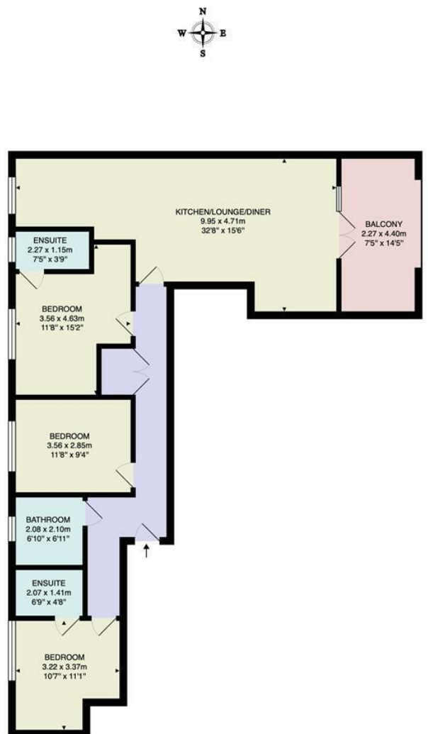
FOURTH FLOOR
